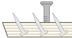
COMS 32mm Architectural Short Pin Carpet Gripper. Available with concrete or wood nails
